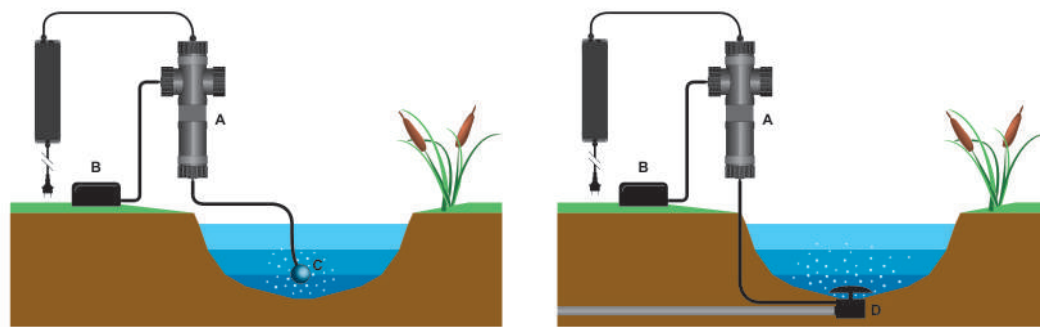
A: FILTREAU OZONE 16W B: AIRPUMP C: AIRSTONE D: BOTTOMDRAIN
